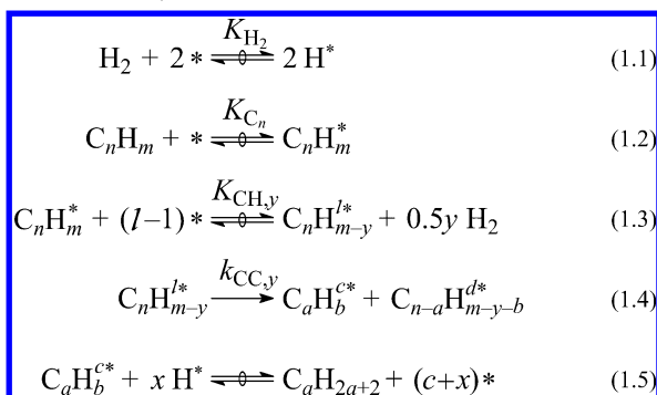
Scheme 1. Proposed Mechanism for Alkane Hydrogenolysis on Metal Catalysts a
