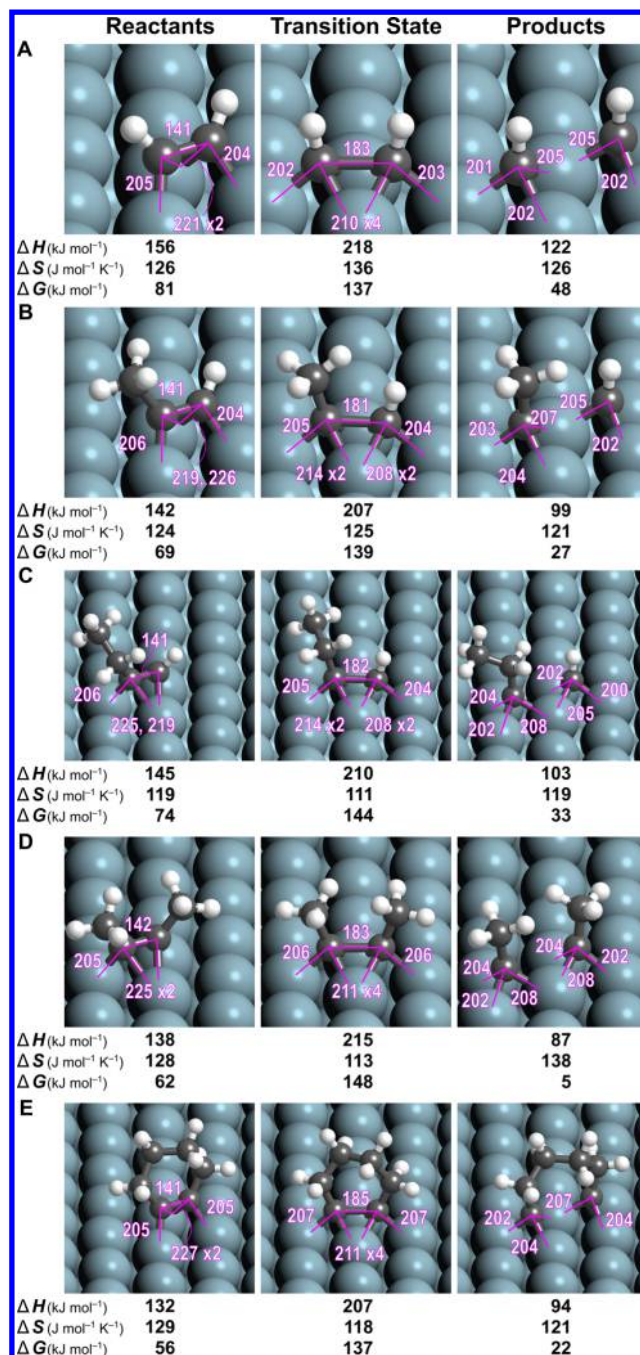
Figure 7. Reactant, transition, and product state structures for C–C activation in RCCR' intermediates derived from (A) ethane, (B) propane, (C and D) butane, and (E) cyclohexane. Shown beneath each image are the \Delta H (kJ mol -1 ), \Delta S (J mol -1 K -1 ), and \Delta G (kJ mol -1 ) values for the formation of each species (and three H 2 (g) molecules) from the alkane reactant and a H*-covered surface.
