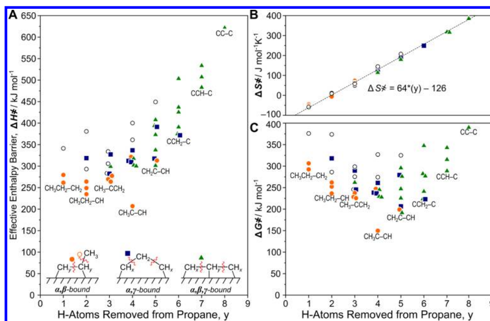
Figure 4. (a) \Delta H^\ddagger , (b) \Delta S^\ddagger , and (c) \Delta G^\ddagger for C–C cleavage of propane-derived intermediates through: \alpha,\beta -bound intermediates via \text{CH}_3\text{CH}_x^*-\text{CH}_y^{\ddagger} ( x = 0-2, y = 0-3 ) (●, orange) and \text{CH}_3^*-\text{CH}_x^*\text{CH}_y^{\ddagger} (○, orange) transition states; \alpha,\gamma -bound intermediates ( \text{CH}_x^*\text{CH}_2\text{CH}_y^{\ddagger} , x = 0-2, y = 0-2 , ■, blue); and \alpha,\beta,\gamma -bound intermediates ( \text{CH}_x^*\text{CH}_y^*\text{CH}_z^{\ddagger} , x = 0-2, y = 0-1, z = 0-2 , ▲, green). The structure of the transition state with the lowest \Delta H^\ddagger and \Delta G^\ddagger is listed near the abscissa for each group with the same number of H atoms removed from propane. Tables S1–S4 in the SI show y, l, \lambda , intrinsic enthalpy barriers ( \Delta H_{\text{act}} ), \Delta H^\ddagger , \Delta S^\ddagger , and \Delta G^\ddagger for each reaction.
