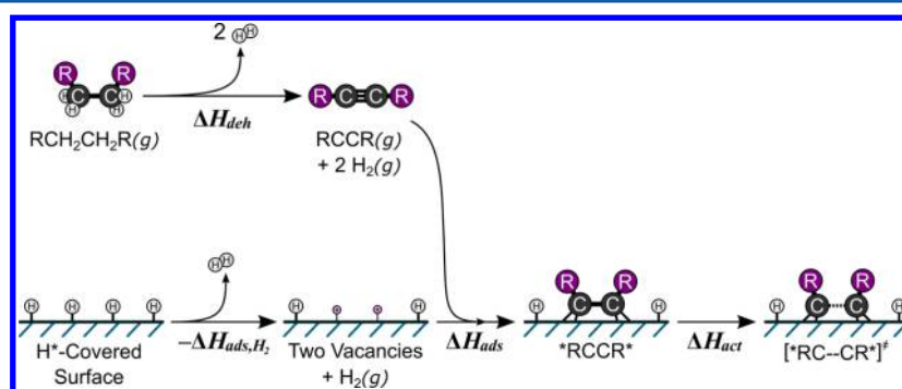
Figure 8. Born–Haber cycle for the formation of the RC–CR' activation transition state.
