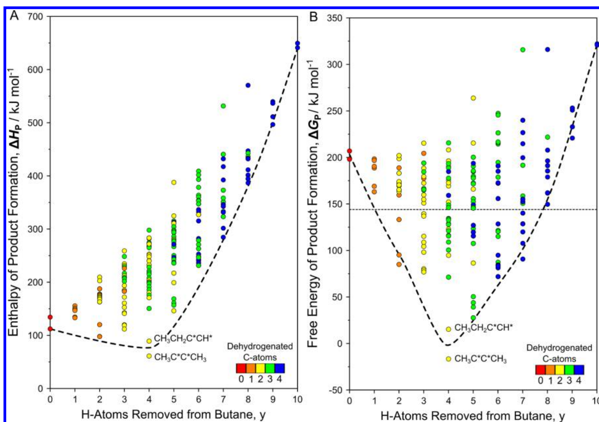
Figure 5. (A) Enthalpy and (B) free energy to form products ( \Delta H_p and \Delta G_p ) of all possible (223) C–C cleavage reactions of C_4 intermediates derived from n -butane. These \Delta H_p and \Delta G_p values represent lower bounds for \Delta H^\ddagger and \Delta G^\ddagger for butane activation. The color of the symbol represents the number of dehydrogenated C atoms (and thus attachments to the surface).
