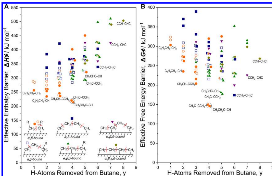
Figure 6. (a) \Delta H^\ddagger and (b) \Delta G^\ddagger values for C–C cleavage in butane-derived intermediates via: \alpha,\beta -bound intermediates (●, orange for activations at \alpha,\beta positions, ○ for activations at \beta,\gamma positions, i.e., between a bound C atom and an unbound C atom); \alpha,\gamma -bound intermediates (□, blue); \alpha,\delta -bound intermediates (■, blue); \alpha,\beta,\gamma -bound intermediates (▲, green); \alpha,\beta,\delta -bound intermediates (▼, purple); and \alpha,\beta,\gamma,\delta -bound intermediates (◆, brown). Notable transition states are labeled.
