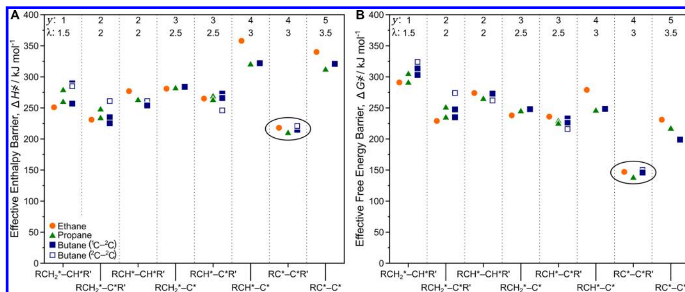
Figure 2. Calculated (A) \Delta H^\ddagger and (B) \Delta G^\ddagger values for C–C bond activation via \alpha,\beta -bound transition states derived from ethane (●, orange), propane (▲, green), and butane ( {}^1\text{C}-{}^2\text{C} , ■, {}^2\text{C}-{}^2\text{C} , □, blue). Within each bin of homologous transition states, points are organized according to alkane reactant. The number of H atoms removed from each transition state (relative to the alkane reactant ( y )) and the total number of \text{H}_2 formed during the formation of each transition state from \text{H}^* -covered surfaces ( \lambda ) are labeled along the top for reference. Table S1 in the SI shows y , l , \lambda , intrinsic enthalpy barriers ( \Delta H_{\text{act}} ), \Delta H^\ddagger , \Delta S^\ddagger , and \Delta G^\ddagger for each reaction.
