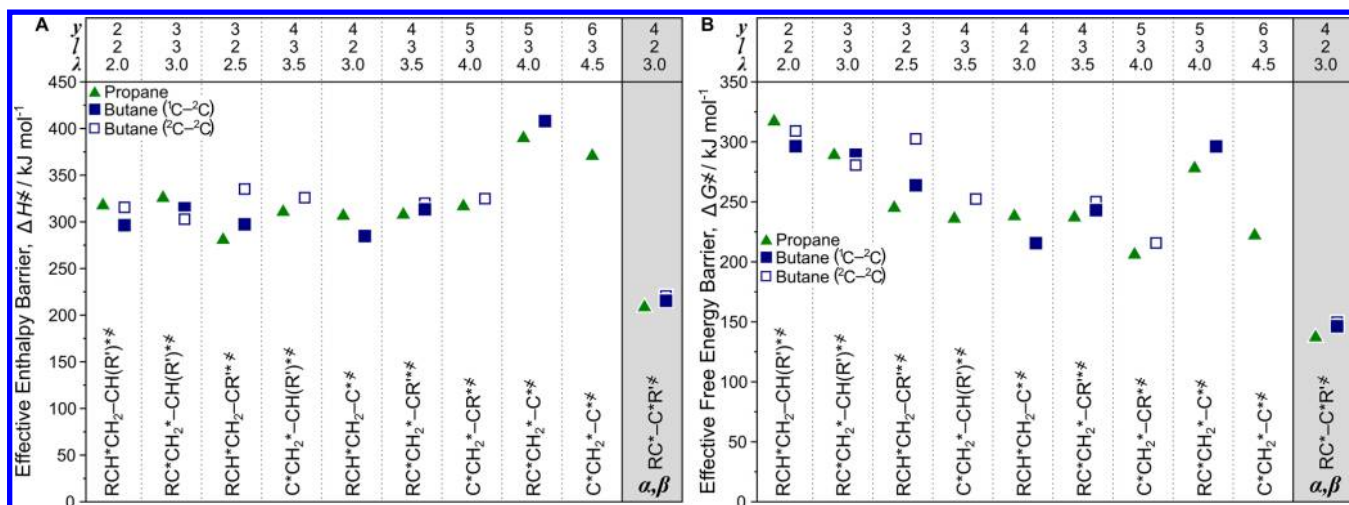
Figure 3. Calculated (A) \Delta H^\ddagger and (B) \Delta G^\ddagger values for C–C bond activation via \alpha,\gamma -bound transition states in propane ( \blacktriangle , green) and butane ( {}^1\text{C}-{}^2\text{C} , \blacksquare , {}^2\text{C}-{}^2\text{C} , \square , blue) (with cleavage via the most favorable \alpha,\beta -bound \text{RC}^*-\text{C}^*\text{R}^\ddagger shown along the far right of each plot for reference). Within each bin of homologous transition states, points are organized according to alkane reactant. The number of H atoms removed from the alkane reagent to form each transition state ( y ), the number of sites required ( l ), and the total number of \text{H}_2 formed during the formation of each transition state from \text{H}^* -covered surfaces ( \lambda ) are labeled along the top for reference. Table S3 in the SI shows y , l , \lambda , intrinsic enthalpy barriers ( \Delta H_{\text{act}} ), \Delta H^\ddagger , \Delta S^\ddagger , and \Delta G^\ddagger for each reaction.
